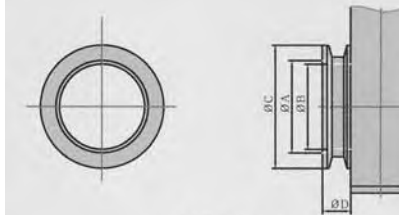
KF Flange
