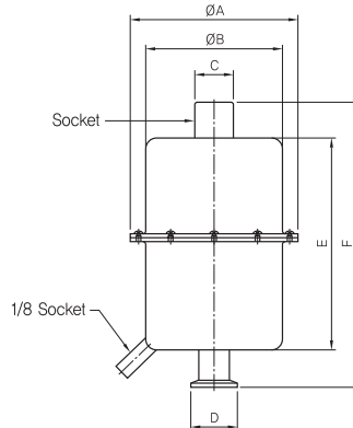
WSO 200~1500
